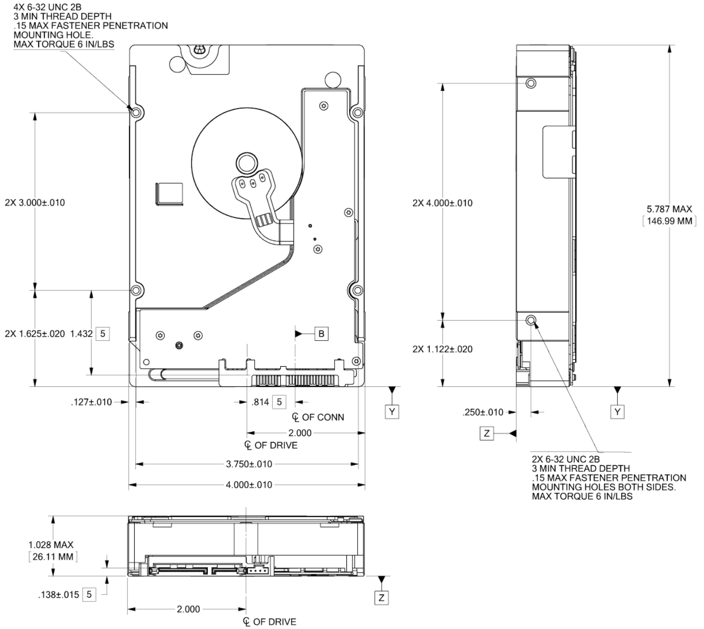
Figure 11. Mounting configuration dimensions (6TB models & ST5000NM0084)
