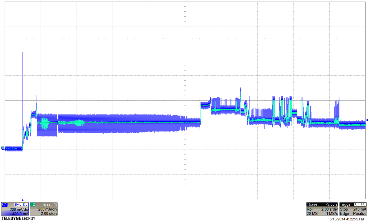
Figure 1. 6TB & ST5000NM0084 Typical 5V startup and operation current profile
