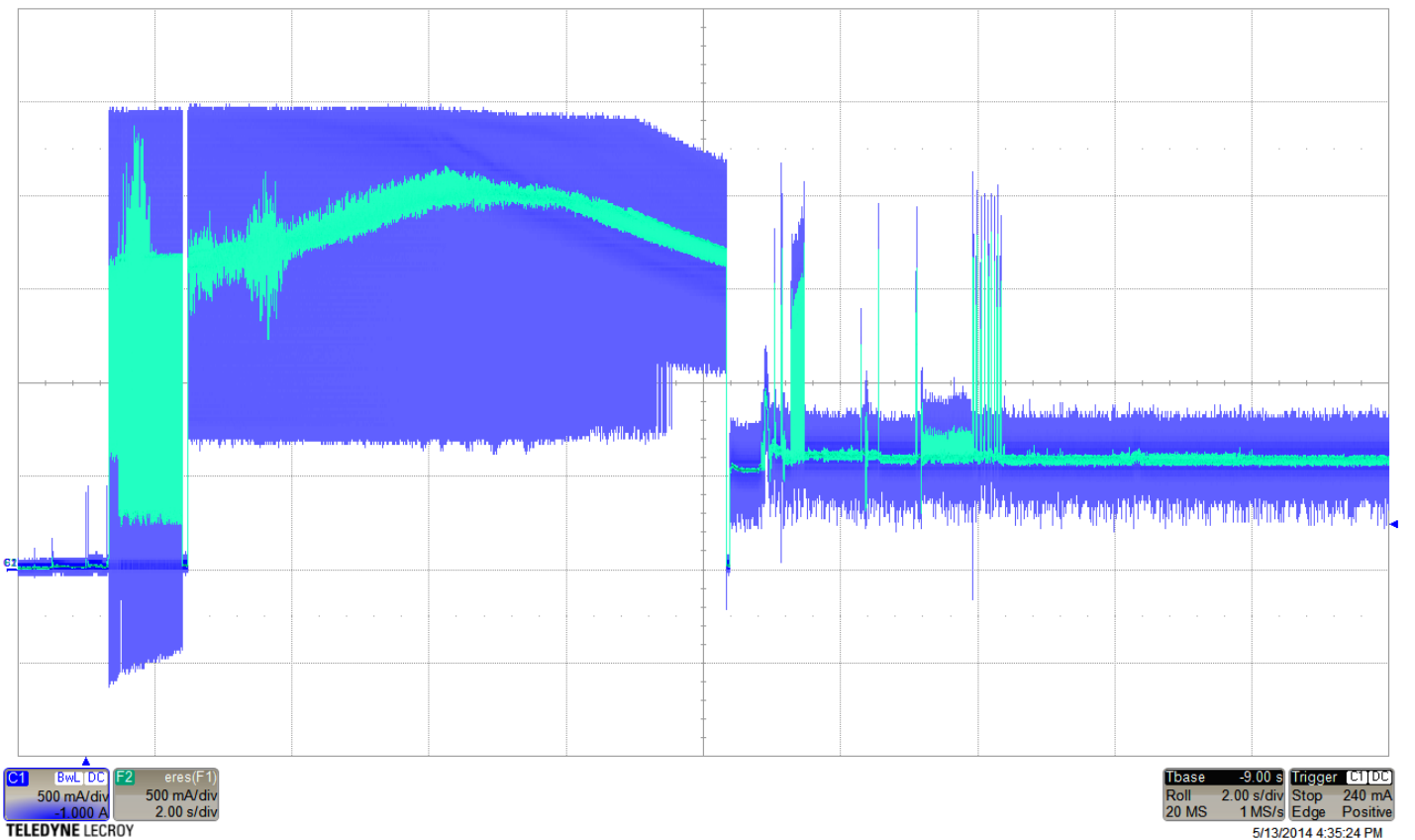
Figure 2. 6TB & ST5000NM0084 Typical 12V startup and operation current profile
