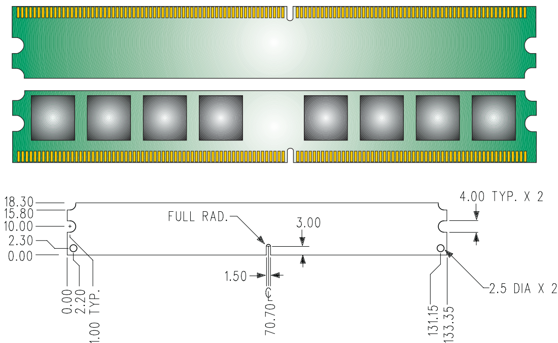
Figure 1: KVR667D2N5/1G 240-Pin DIMM
