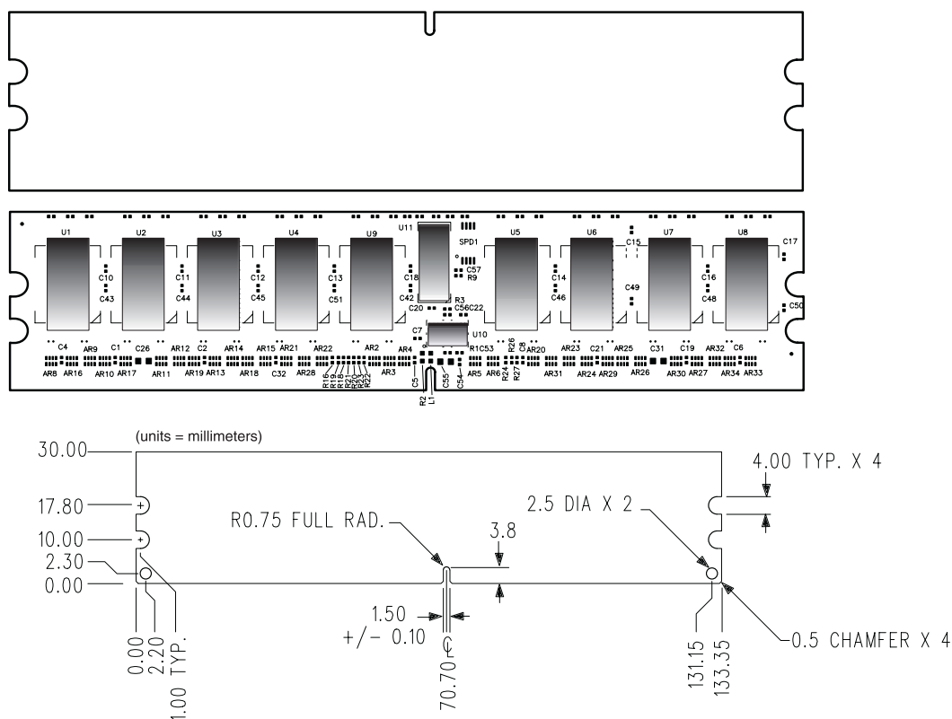
Figure 1: KVR400D2S8R3/1GI 240-Pin DIMM
