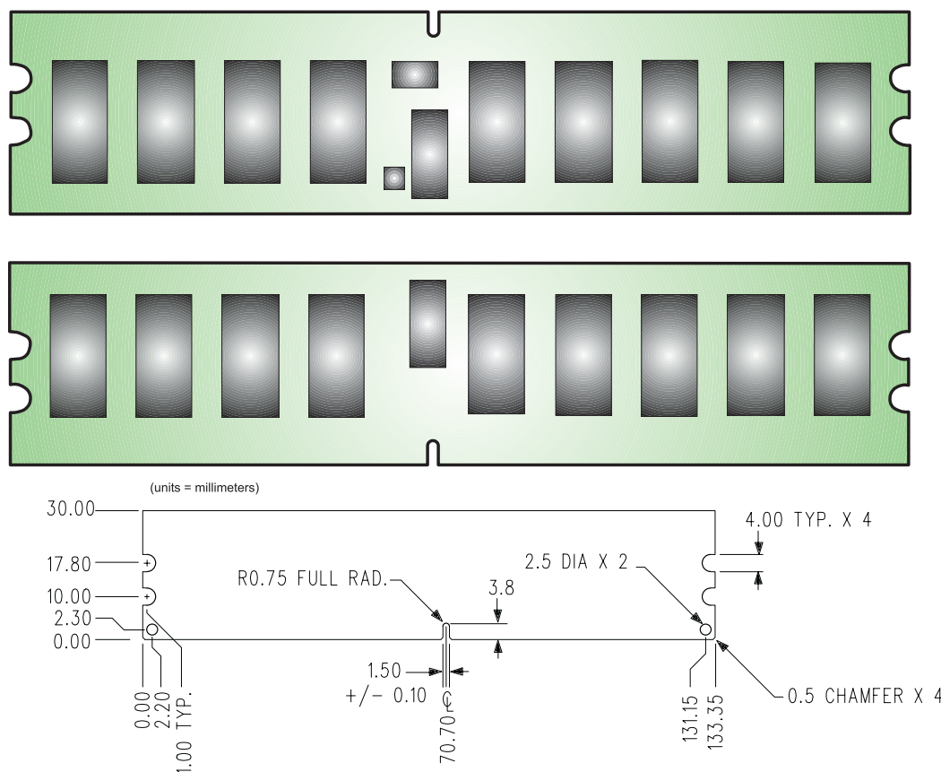
Figure 1: KVR800D2S4P6K2/4G 240-Pin DIMM
