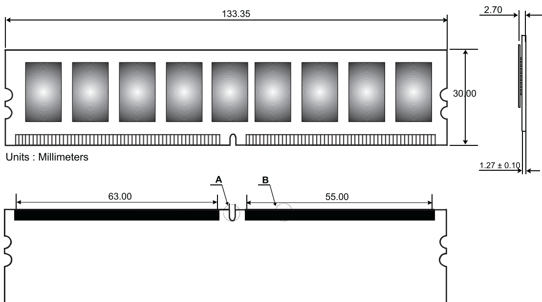
Figure 1: KVR533D2E4/1G 240-Pin DIMM
