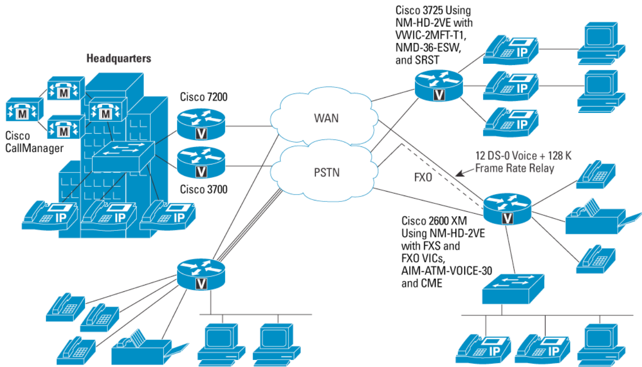
Figure 2. IP Telephony Application using Cisco CallManager Express and SRST in the Business Branch
